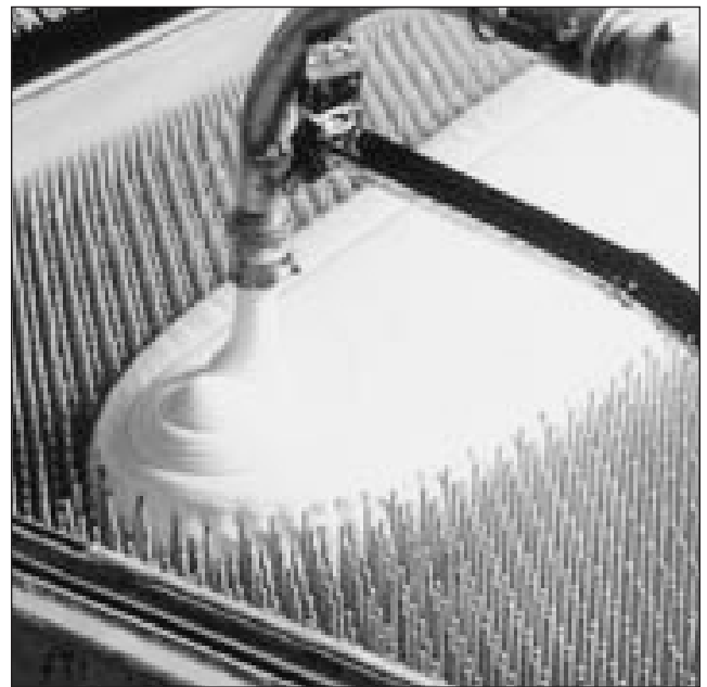
Filling a Talalay mold with latex suspension
